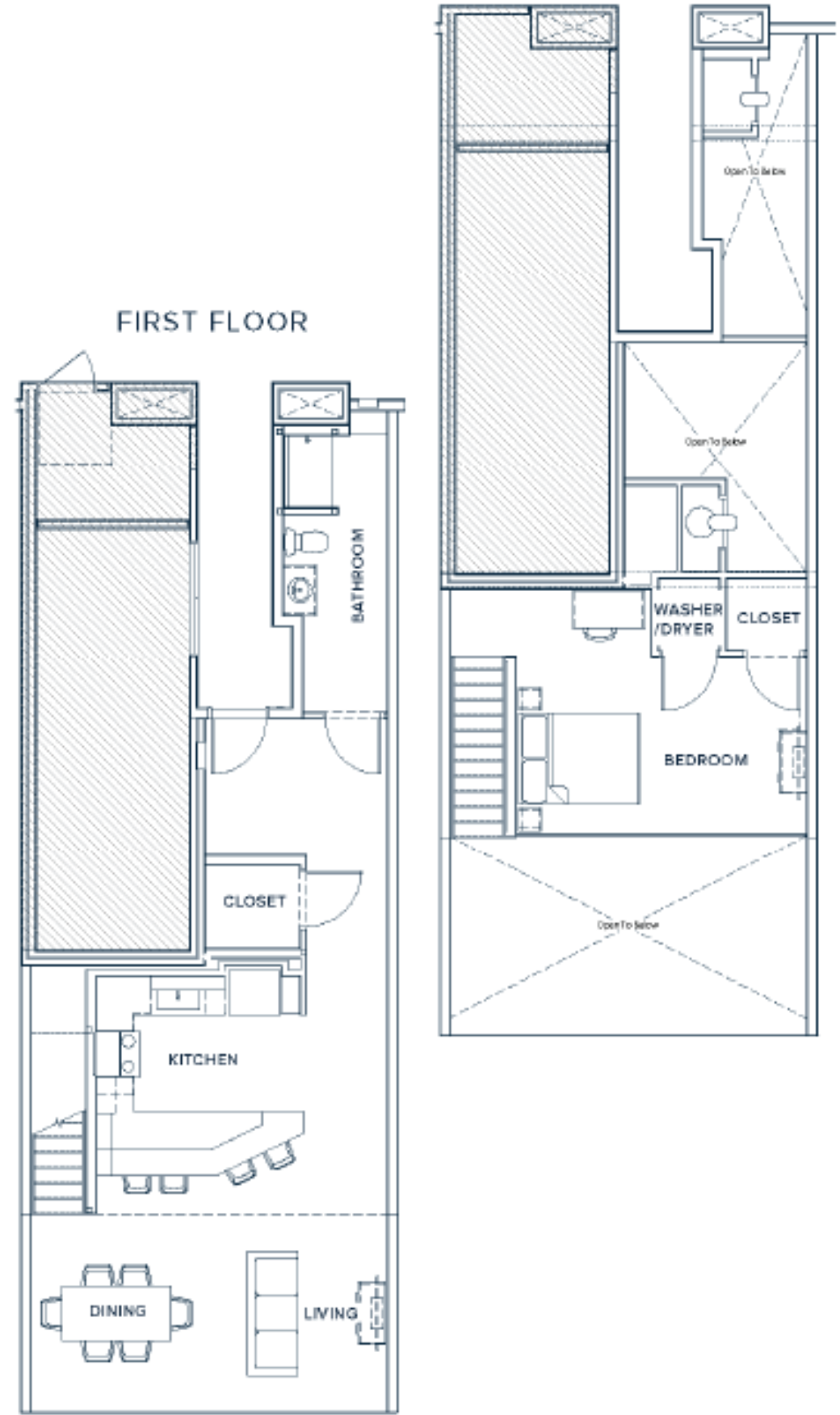
SECOND FLOOR
